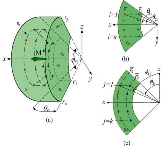
Fig. 10. Customized PM geometry ( r_o = 46.5 mm, r_i = 23 mm, \theta_o = 40^\circ , \phi_o = 70^\circ ; \mu_o M_o = 0.62 T). (a), (b) n = 5 , (c) k = 11 .
