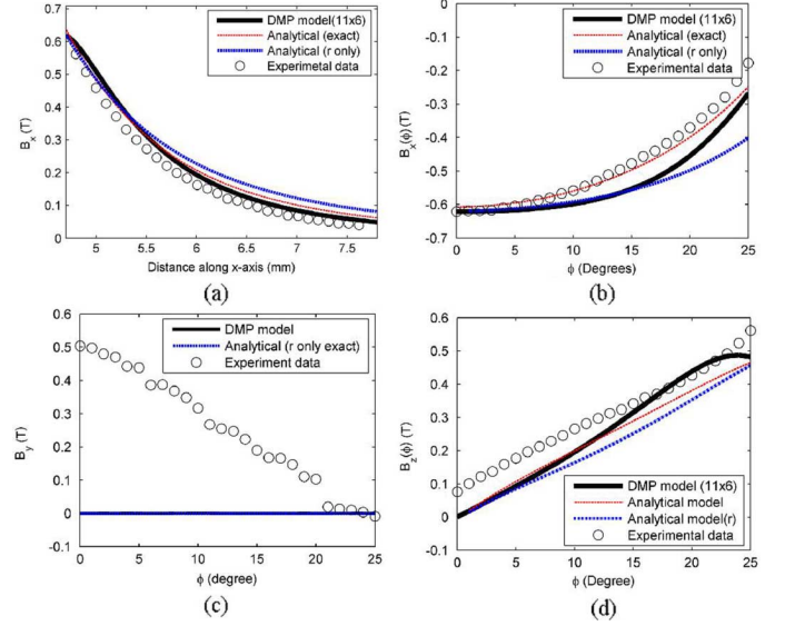
Fig. 11. Comparisons of magnetic flux density. (a) x -axis, (b) B_x(\phi) , (c) B_y(\phi) , (d) B_z(\phi) .
