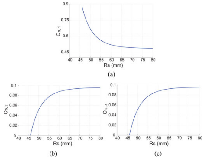
Fig. 2. Relationship between flux density and stator radius ( r = 46.5 mm). (a) O_{s,1} versus R_s . (b) O_{s,2} versus R_s . (c) O_{s,3} versus R_s .
